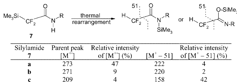
Scheme 8. Thermal behavior of 7 and relative magnitude of the loss of the \text{CHF}_2 fragment.
