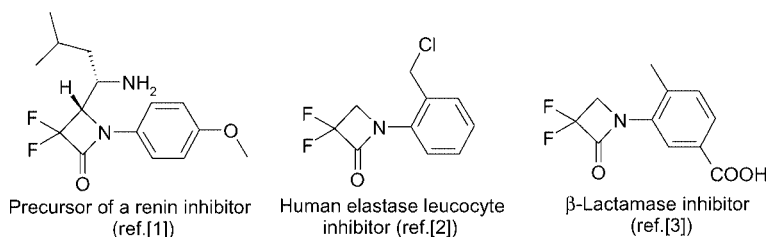
Scheme 1. Bioactive 3,3-difluoroazetidin-2-ones.
